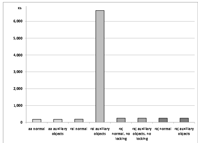
Figure 10. Memory consumption in Kilobytes for association aspects (aa), relationship aspect library (ral) and relational aspects (raj, with and without locking)
