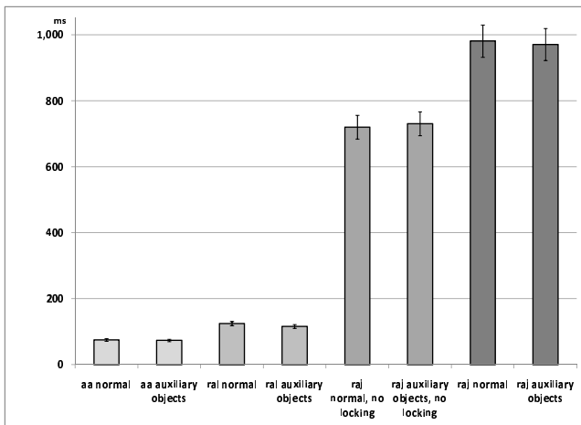
Figure 9. Running times in milliseconds for association aspects (aa), relationship aspect library (ral) and relational aspects (raj, with and without locking)
